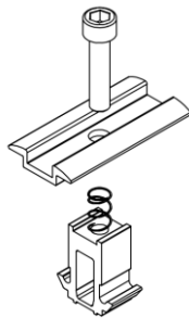
Kit MiniClamp MC 30-50 mm
